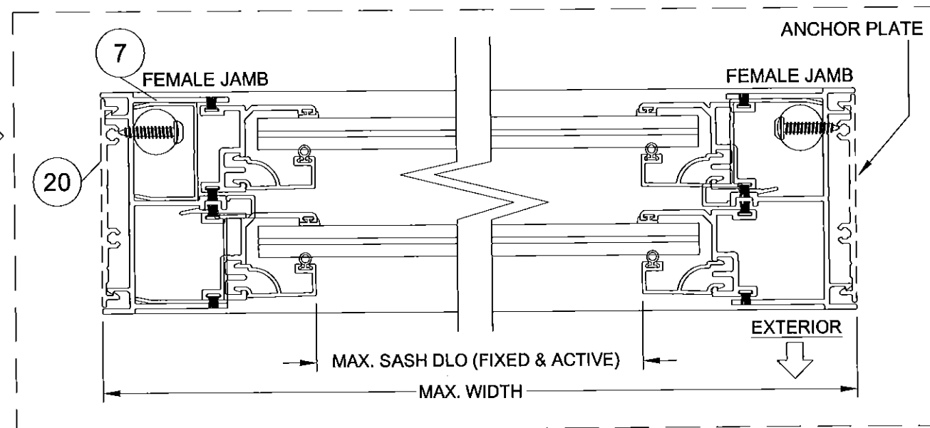
ALT. SECTION B-B OPTIONAL ANCHOR PLATE & FEMALE JAMB
